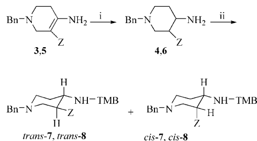
Scheme 2. Reagents and conditions: 3,4,7 : \text{Z} = \text{CO}_2\text{Et} , 5,6,8 : \text{Z} = \text{CN} . (i) for 4 : \text{NaBH}_3\text{CN} , EtOH, HCl, 50 °C, 3 h, 65%; for 6 : \text{NaBH}_3\text{CN} , EtOH, HCl, 50 °C, 12 h, 81%; (ii) for cis - and trans - 7 : TMB-Cl, \text{NEt}_3 , \text{CH}_2\text{Cl}_2 , room temp., 4 h, 56.3 and 30.4%, respectively; for cis - and trans - 8 : TMB-Cl, \text{NEt}_3 , THF, room temp., 1 h, 50 and 36%, respectively.
