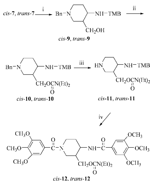
Scheme 3. Reagents and conditions: (i) \text{NaBH}_4 , \text{LiCl} , THF, EtOH, room temp., 36 h, 57 and 83%, respectively; (ii) \text{NaH} , THF, \text{ClCON}(\text{Et})_2 , reflux, 90 min, 81 and 93%, respectively; (iii) \text{Pd}/\text{C} , \text{HCO}_2\text{NH}_4 , MeOH, reflux, 1 h, 81 and 43%, respectively; (iv) 3,4,5- (\text{CH}_3\text{O})_3\text{C}_6\text{H}_2\text{COCl} , \text{NEt}_3 , THF, room temp., 90 min, 88 and 71%, respectively.
