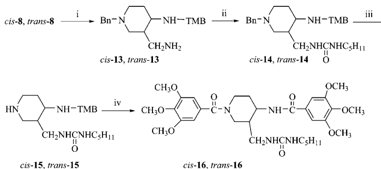
Scheme 4. Reagents and conditions: (i) \text{H}_2 , \text{Ni} , EtOH, concd. \text{HCl} (cat.), 60 °C, 12 h, 75 and 37%, respectively; (ii) \text{C}_5\text{H}_{11}\text{N}=\text{C}=\text{O} , \text{CH}_2\text{Cl}_2 , room temp., 2 h, 65%; (iii) \text{Pd}/\text{C} , \text{HCO}_2\text{NH}_4 , MeOH, reflux, 1 h, 79 and 60%, respectively; (iv) 3,4,5- (\text{CH}_3\text{O})_3\text{C}_6\text{H}_2\text{COCl} , \text{NEt}_3 , THF, room temp., overnight, 61 and 74%, respectively.
