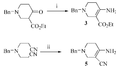
Scheme 1. Reagents and conditions: (i) \text{AcONH}_4 , MeOH, room temp., 1 h, 99%; (ii) \text{NaNH}_2 , THF, reflux, 2 h, 81%.
